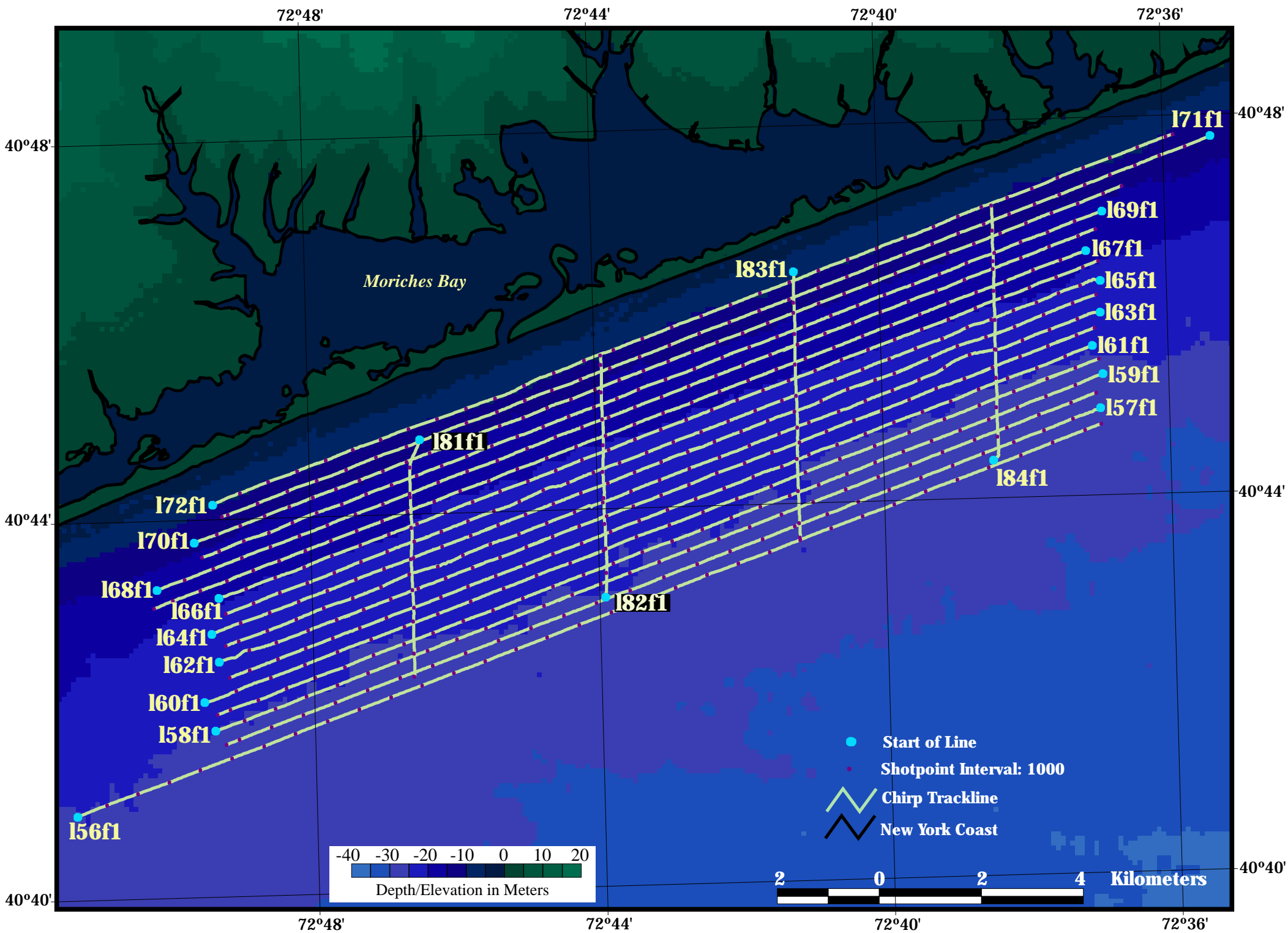
DIAN 97011 Chirp Survey Area 4 (Lines 56-72, 81-84)
