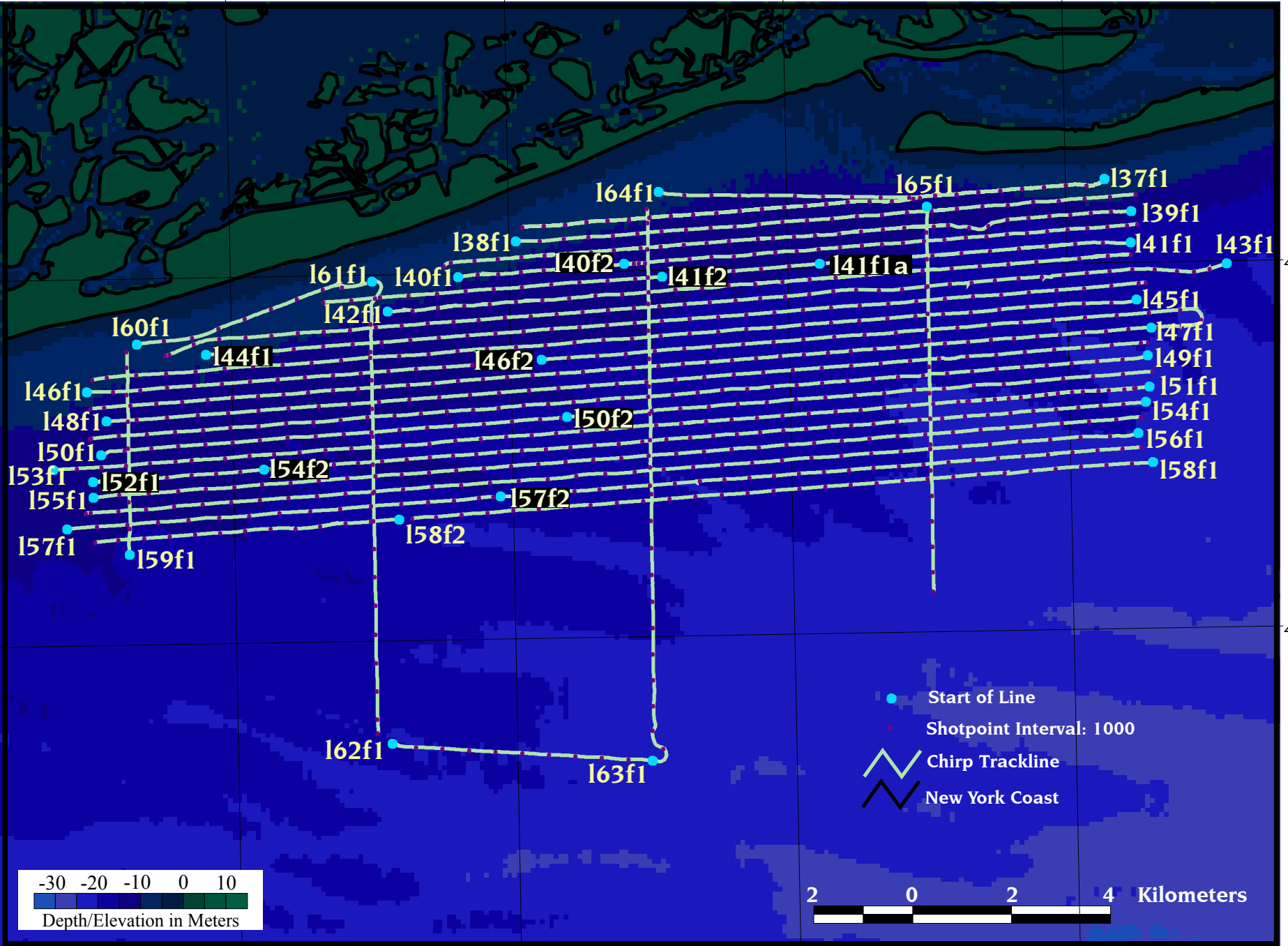
DIAN 96040 Chirp Survey Area 1 (Lines 37-65)
