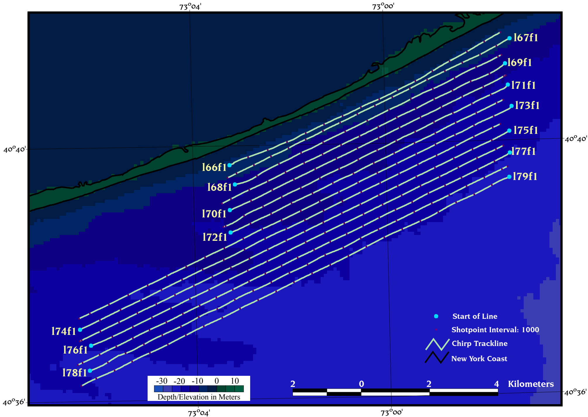
DIAN 96040 Chirp Survey Area 3 (Lines 66-79)
