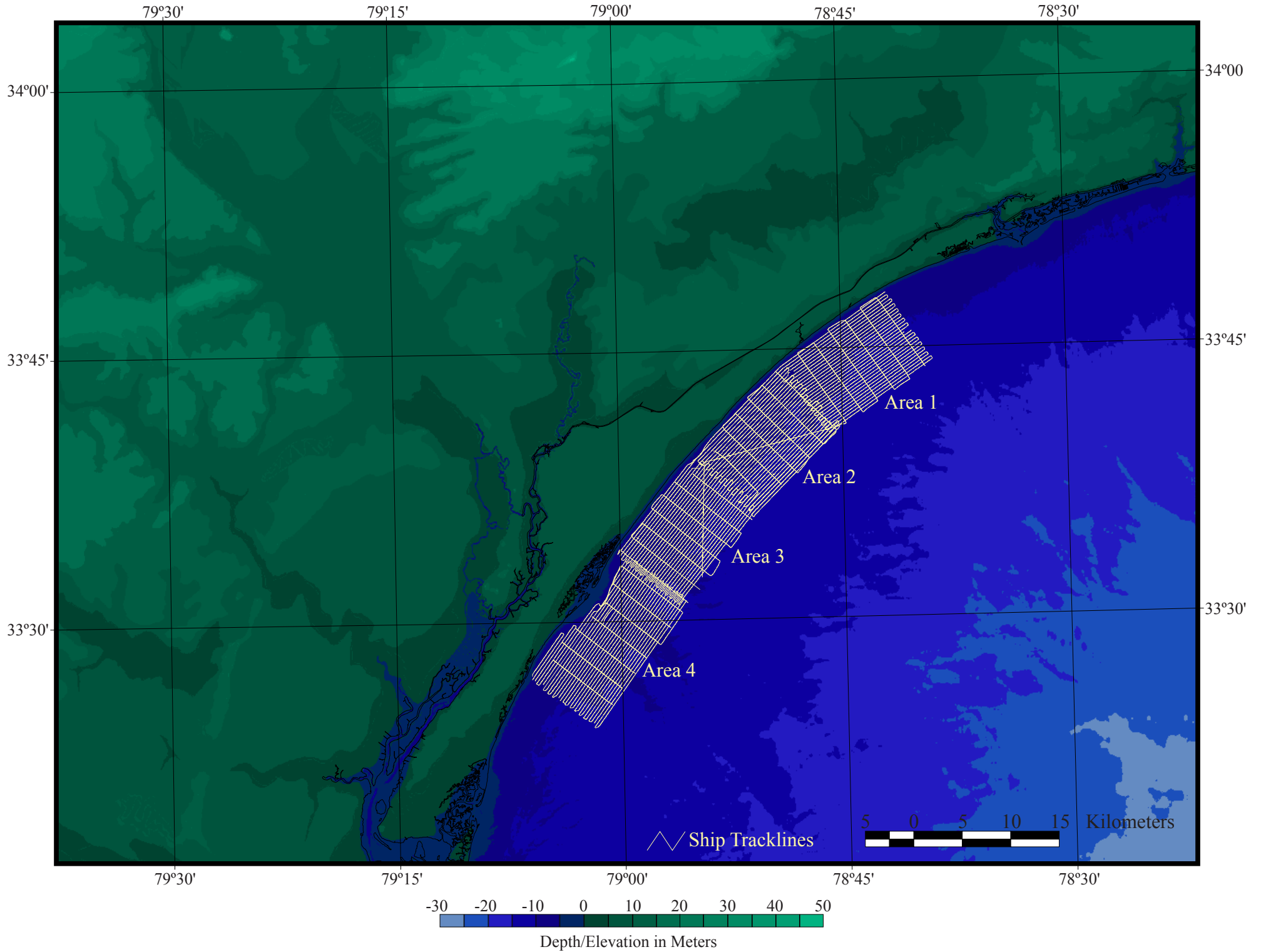
ATSV 99044 Full Extent of Chirp Survey Area
