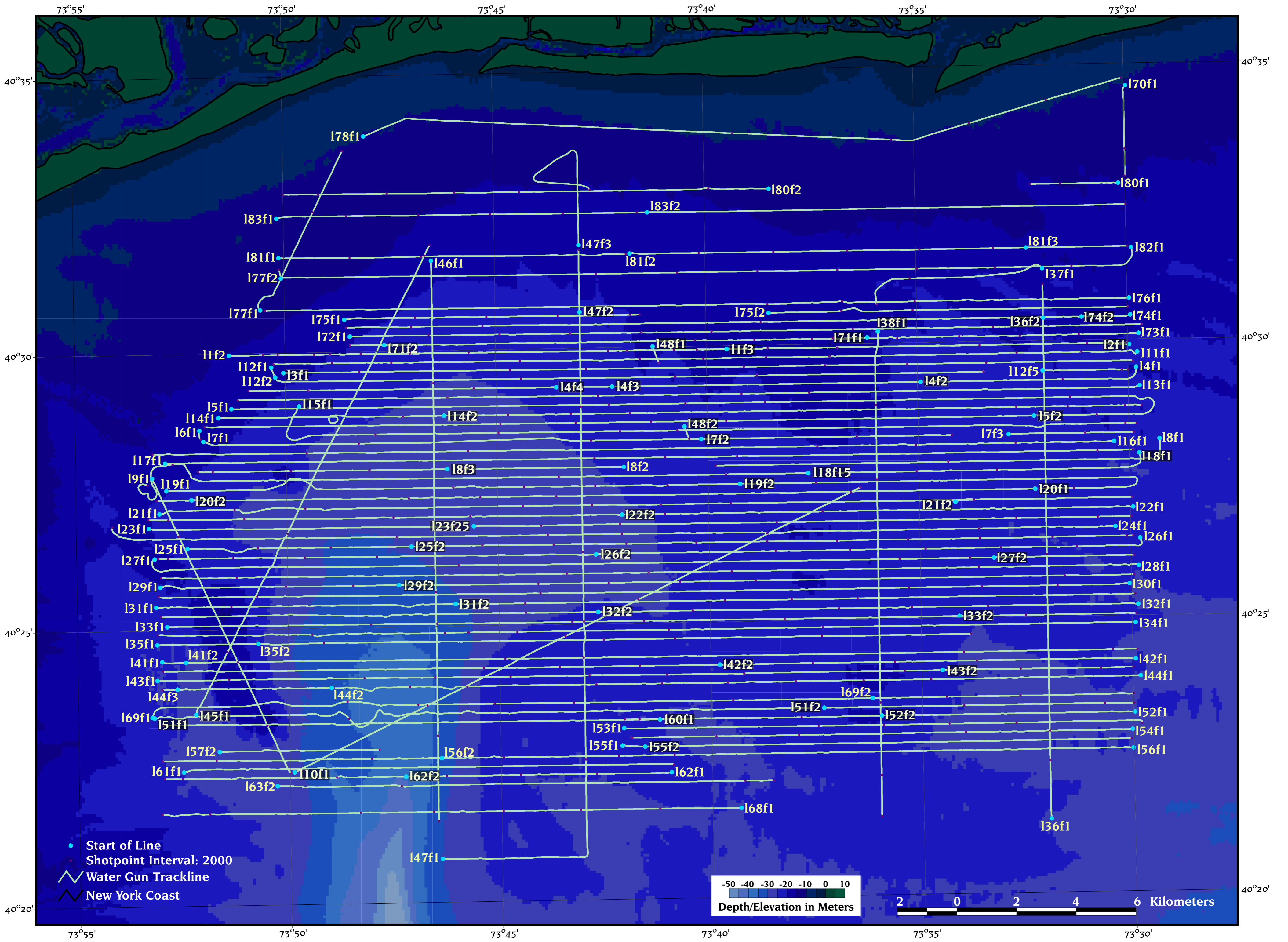
Full Extent of SEAX 95007 Water Gun Survey Area
