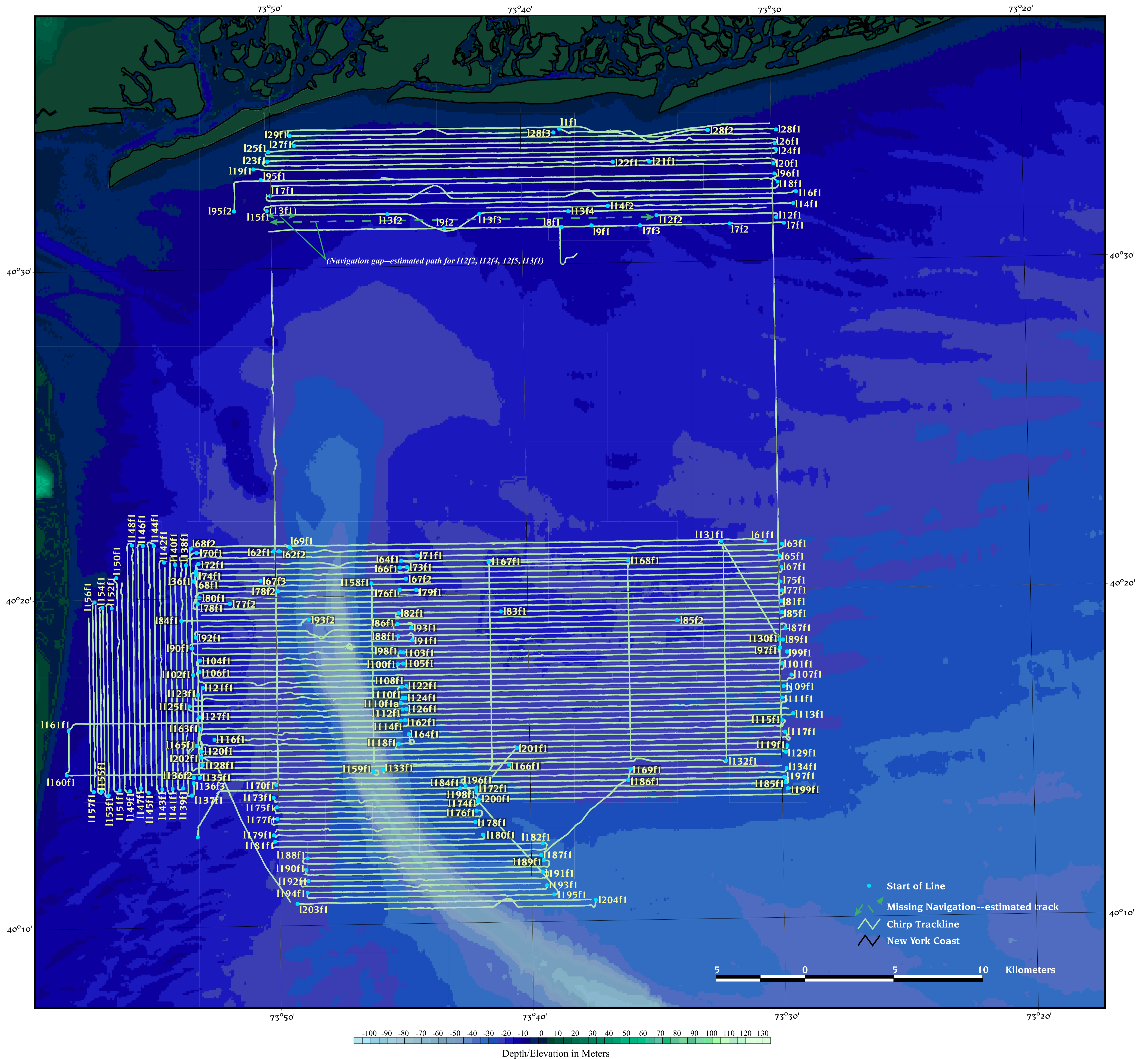
SEAX 96004 New York Bight Sidescan-Sonar Mosaic Area (lines 1-29, 61-204)
