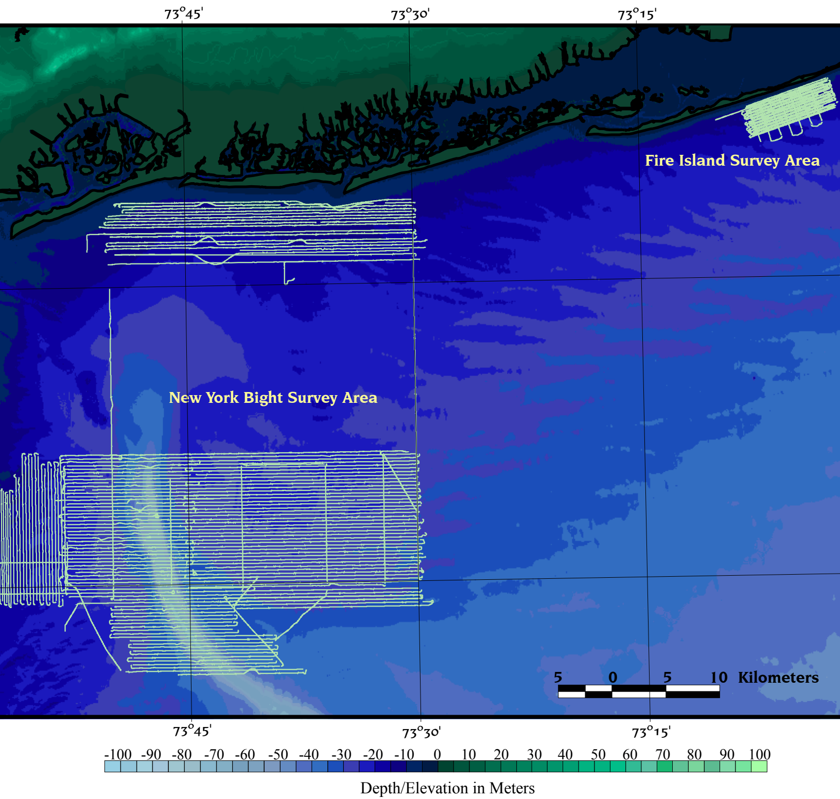
Full Extent of SEAX 96004 Sidescan Mosaic Area
