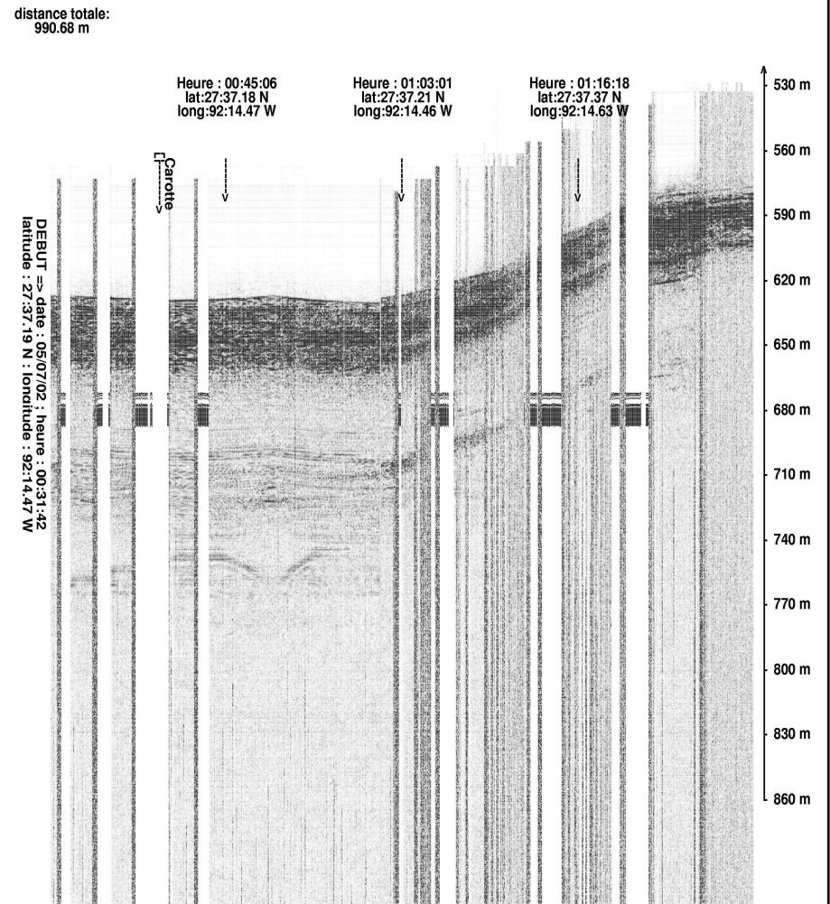
MD02-2536G Coring Operation
