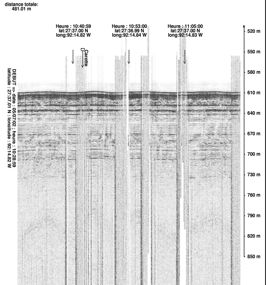
MD02-2538G Coring Operation
