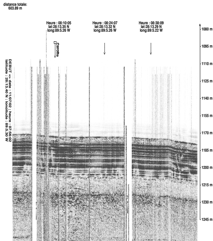
MD02-2559 Coring Operation
