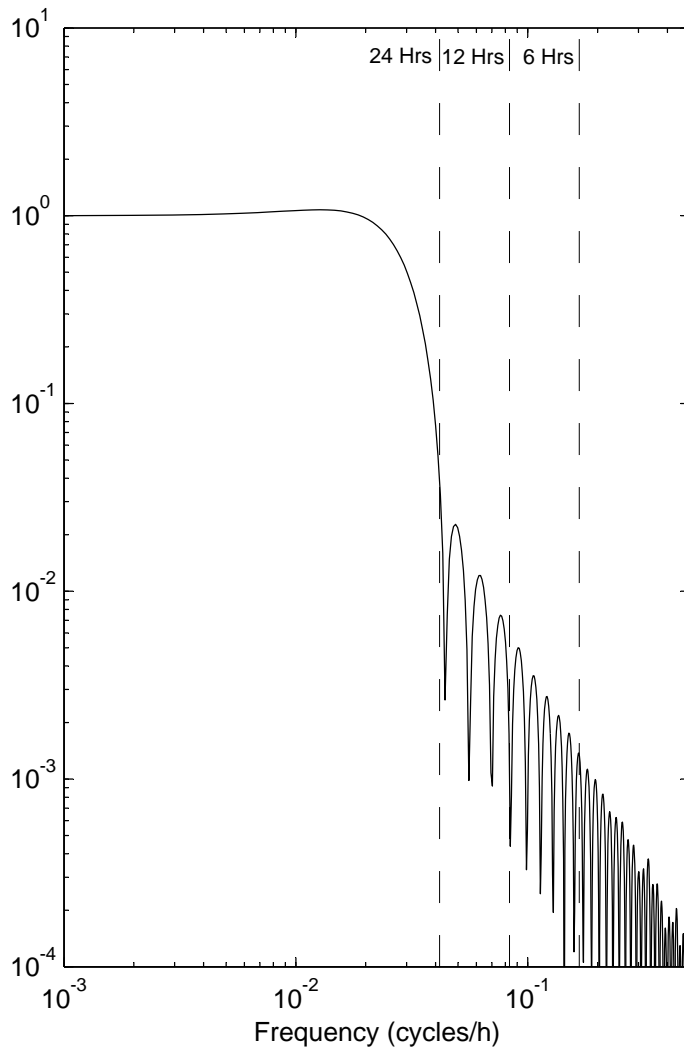
Figure 48: Amplitude transfer function for the low-pass filter PL33, showing the amplitude response as a function of frequency.
