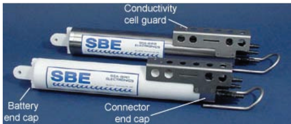
Figure 24. A photograph of the SEACAT 16 conductivity and temperature sensor manufactured by Sea-Bird Electronics. The temperature and conductivity sensors are located under the conductivity cell guard. This photo is courtesy of Sea-Bird Electronics.
