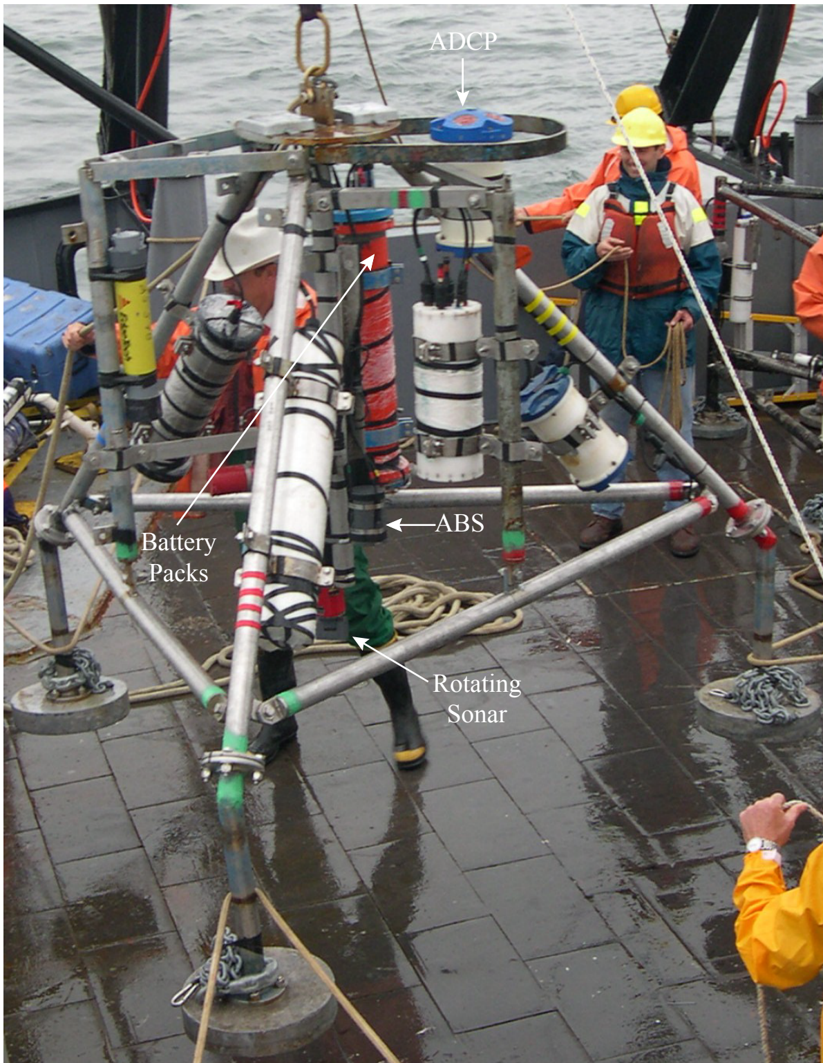
Figure 13. A photograph of a tripod being deployed from the Research Vessel Dan Moore at site 7B. Instruments on this tripod included an Acoustic Doppler Current Profiler (ADCP), Acoustic Backscatter Sensor (ABS), and a rotating sonar.
