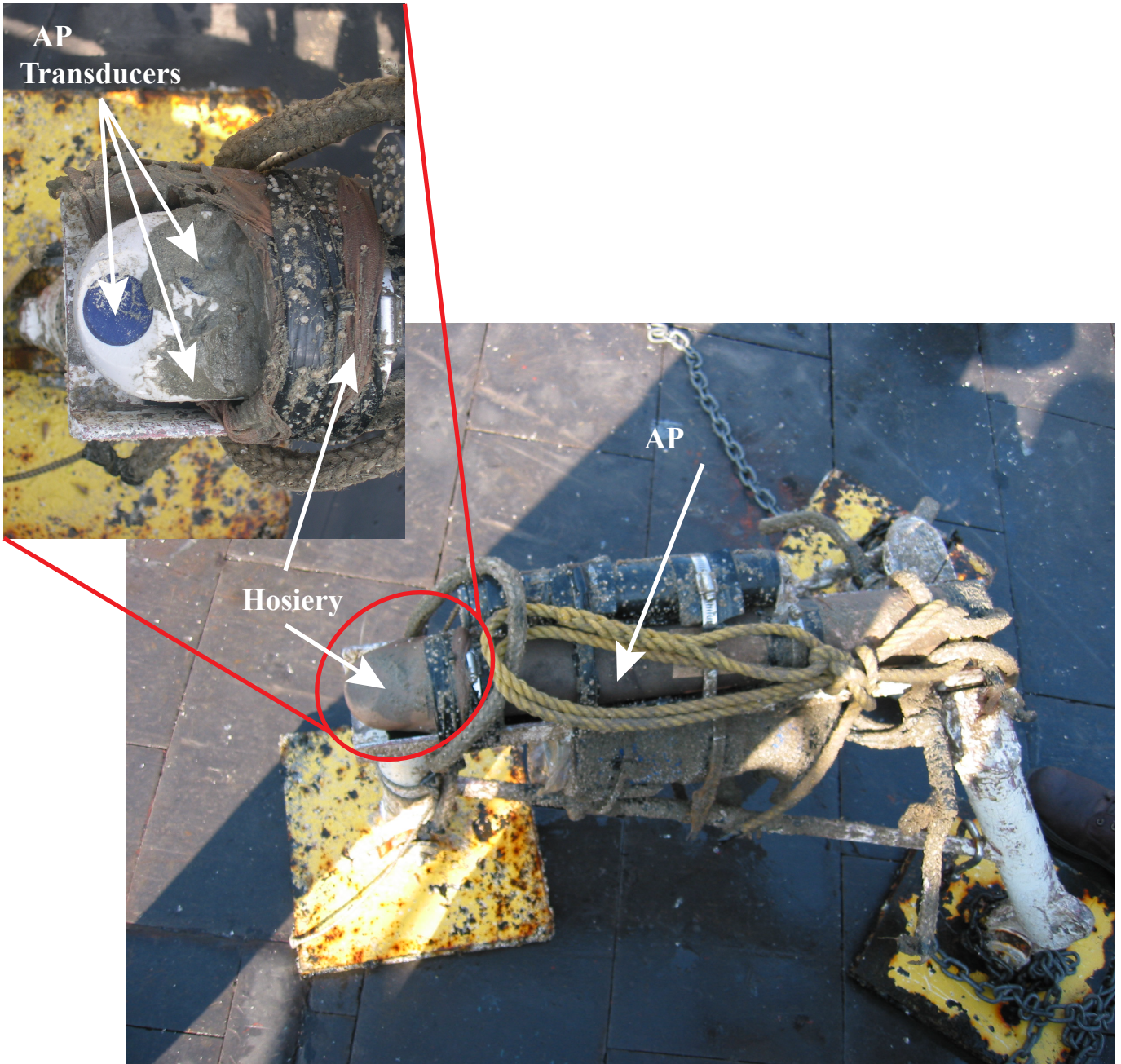
Figure 46. A photograph of the tripod recovered from Site 8 at the end of the second deployment. The tripod surface and the surface of the AP are not significantly biofouled. However, upon removal of the hosiery (used to prevent biofouling), two of the three transducers on the AP were covered with mud.
