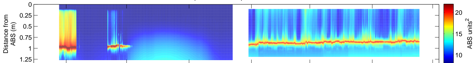
Squared Mean Amplitude at 5 Mhz
