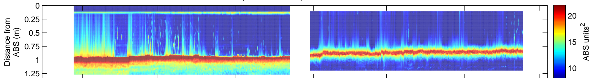
Squared Mean Amplitude at 2.5 Mhz
