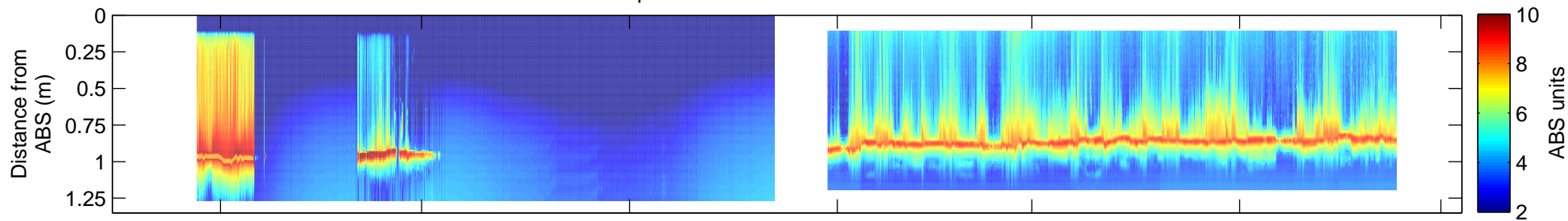
Amplitude Standard Deviation at 5 Mhz
