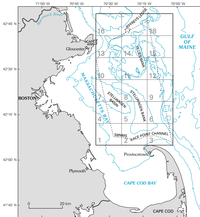
Location map showing regional setting of the map area (outlined in black) and locations of quadrangles. Stellwagen Bank National Marine Sanctuary (SBNMS) boundary is shown as a dashed line. Bathymetric contours are labeled in meters.
