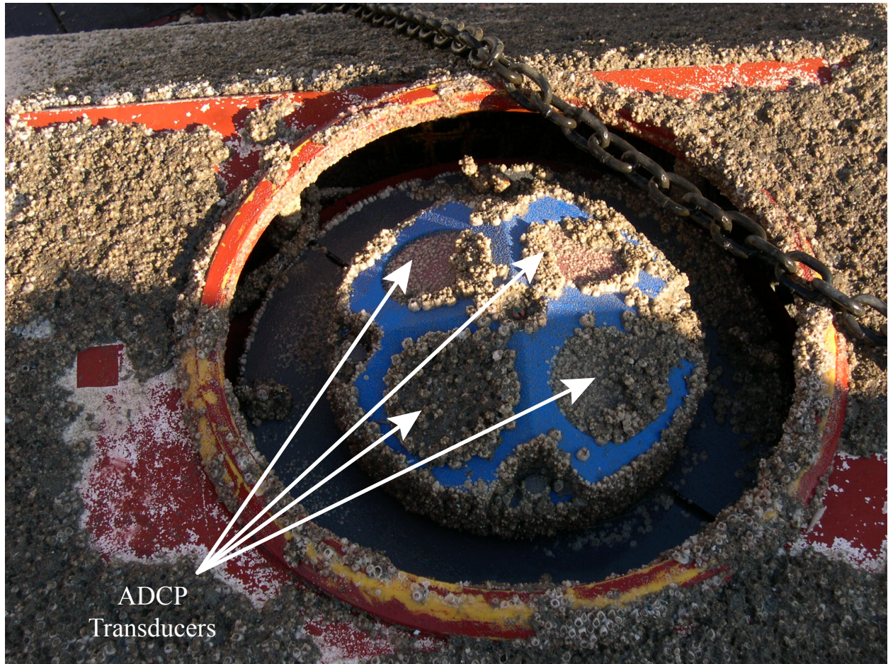
Figure 36. A photograph of the TRBM and the ADCP recovered from Site 4 at the end of the first deployment. Both the TRBM and ADCP transducers are heavily biofouled.
