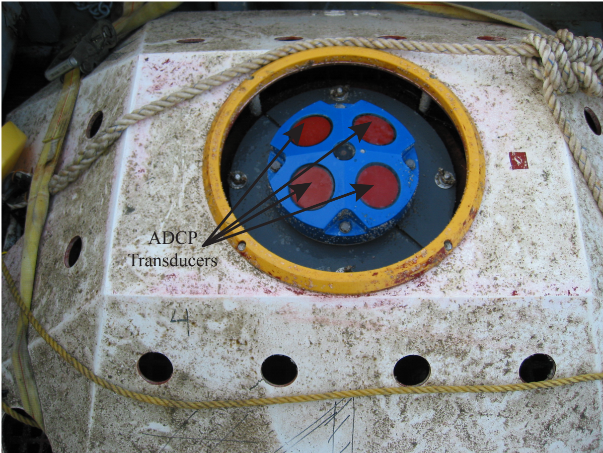
Figure 37. A photograph of the TRBM and ADCP recovered from Site 4 at the end of the second deployment. The ADCP transducers were mostly free from biofouling.
