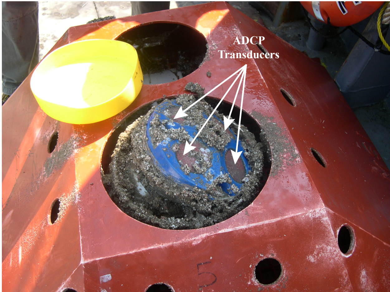
Figure 38. A photograph of the TRBM and ADCP recovered from Site 5 at the end of the second deployment. This instrument package was not recovered and cleaned at the end of the first deployment. The ADCP was therefore in the water for the entire 6-month duration. Biofouling of the ADCP during this time was significant. The ADCP also became tilted, which led to the complete loss of data at this site.
