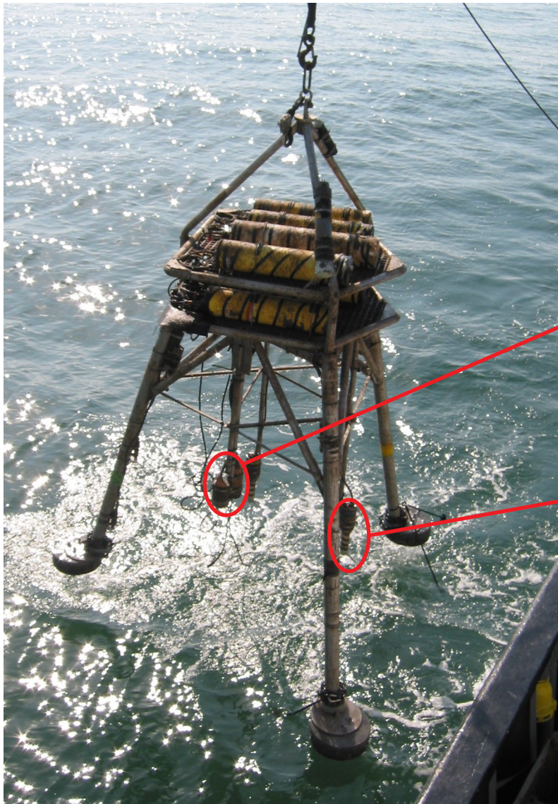
Figure 42. Photographs of the tripod and instruments recovered at Site 7A at the end of the second deployment. Biofouling was not as significant during this deployment.
